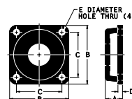
FLANGE BRACKET
