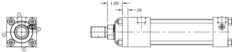
SERIES TS/TSM (1 1/2 BORE oversized rod)
